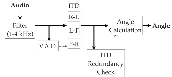
Fig. 3. Initial DOA Estimation flow of data.
