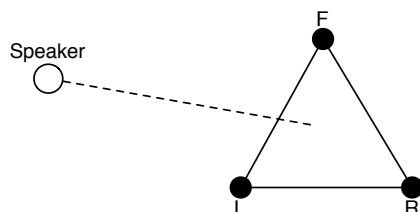
Fig. 2. Hardware setup of the proposed system.
