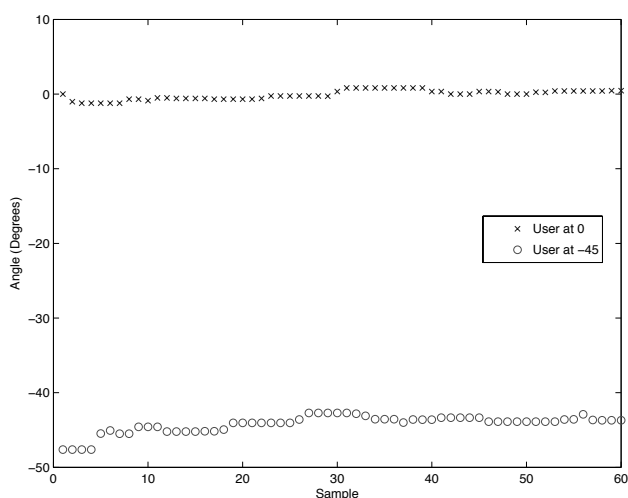
Fig. 5. Tracking 2 simultaneous sources (2 electronic speakers).
