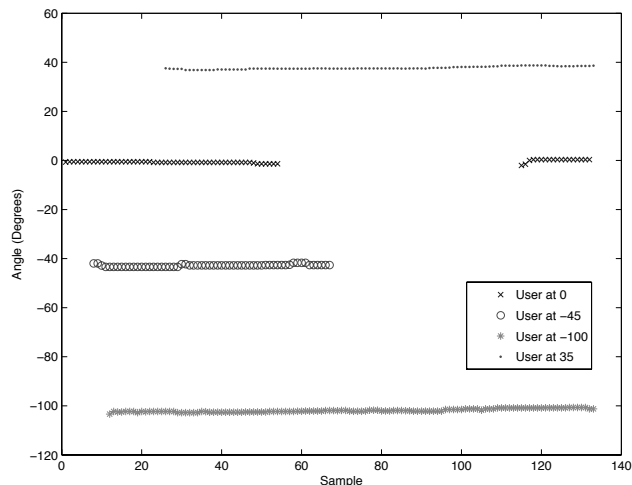
Fig. 7. Tracking 4 simultaneous sources (2 electronic speakers, 2 humans).
