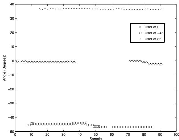
Fig. 6. Tracking 3 simultaneous sources (2 electronic speakers, 1 human).
