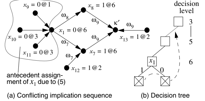
Figure 3: Non-chronological backtracking
