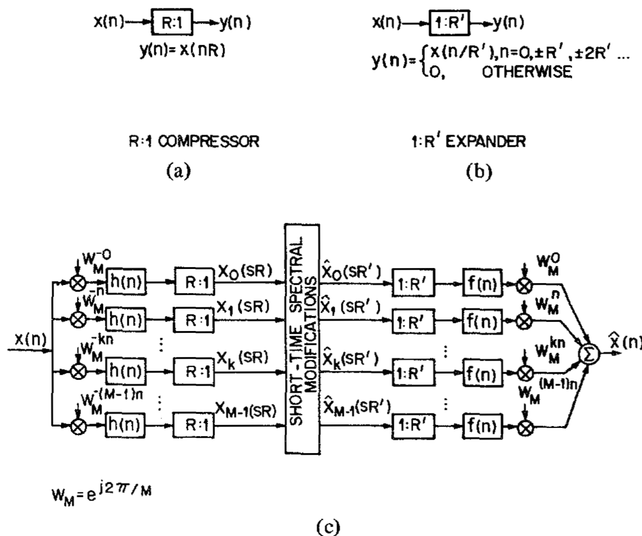
Fig. 3. The filter-bank summation interpretation of short-time Fourier analysis/synthesis.
